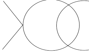
Figure 1: Simple example of diagram that generates an extra subdivergence
