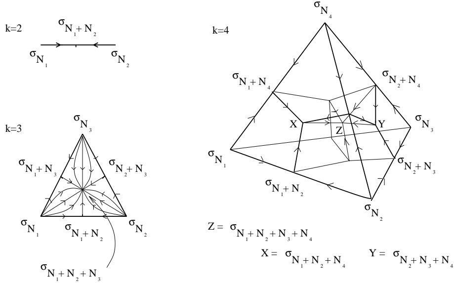
Figure 3: Polyhedral RG patterns interpolating between pairs of \sigma_N models.
