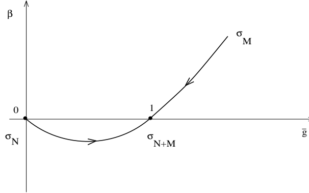
Figure 2: Beta function of dual RG flows.
