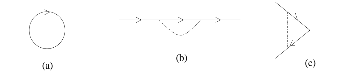
Figure 1: Leading diagram and first subleading corrections.
